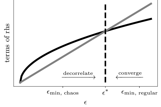
Figure 4. Fixed-point average distance between replica implies chaotic-subspace. The square root term \propto \sqrt{\epsilon} (black curve) and the linear term \propto \epsilon in (13) intersect and produce a fixed point \epsilon^* for the covariance Q_0 - \epsilon between the two replicas. The resulting average Hamming distance d^* between states in the two copies of the system is given by \epsilon^* and (16) as d^* = N\epsilon^*/g^2 . Depending on whether \epsilon_{\text{min}} (which corresponds to a Hamming distance of d_{\text{min}} = 1 ) is smaller or larger than \epsilon^* , the replicas will either decorrelate, or they will converge and forget the perturbation.
